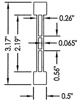
2 MULLION (5902) 6105-T5 ALUM
