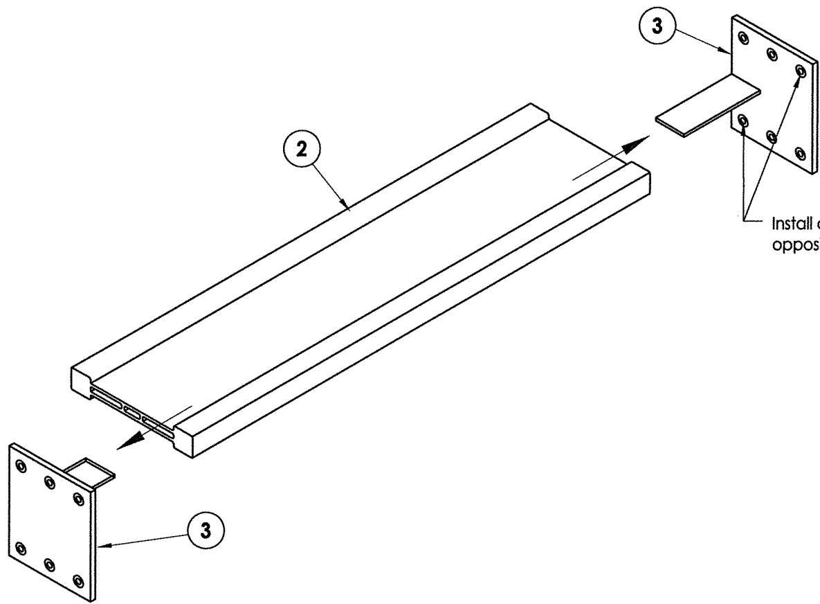
BRACKET TO MULLION DETAIL
