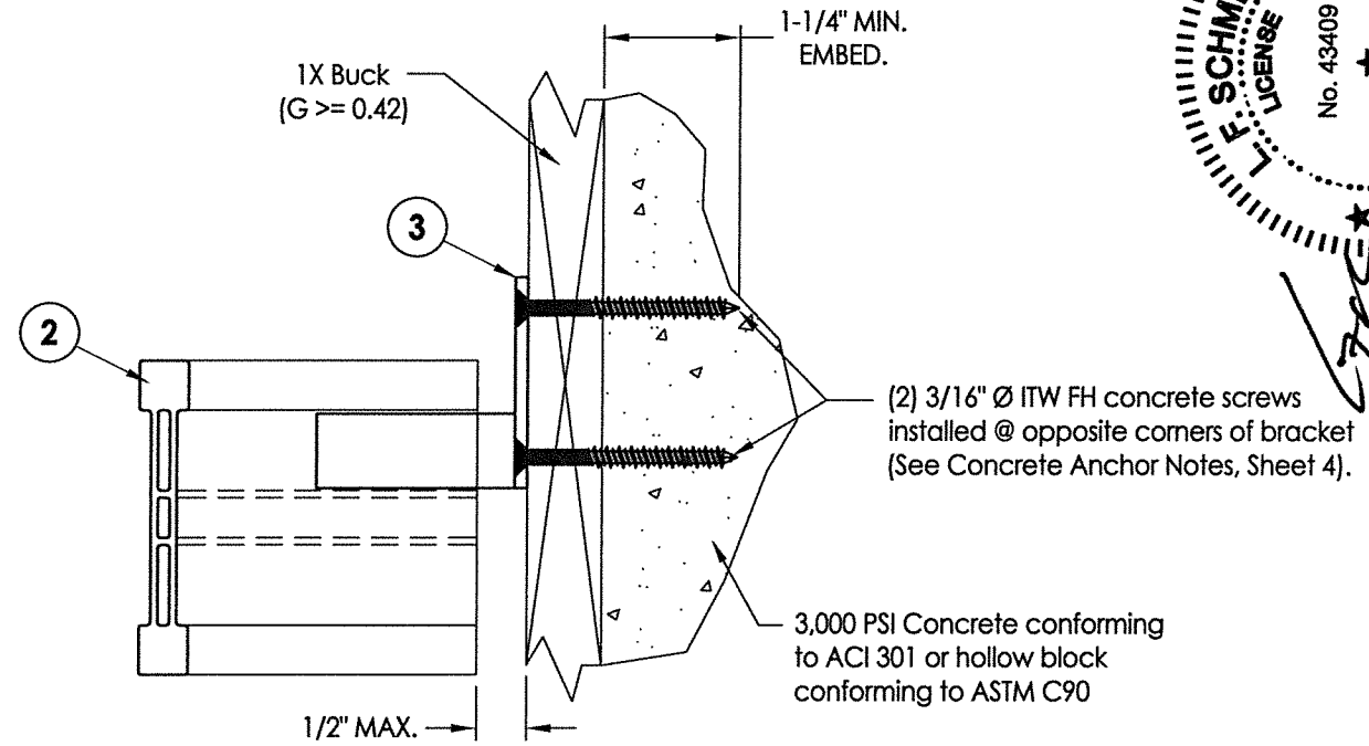
2 ANCHOR BRACKET DETAIL 3 Anchor to masonry thru 1x buck
