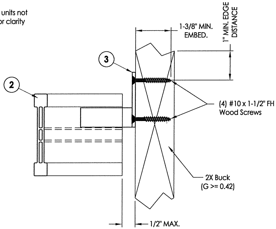
1 ANCHOR BRACKET DETAIL 3 Anchor to 2x buck
