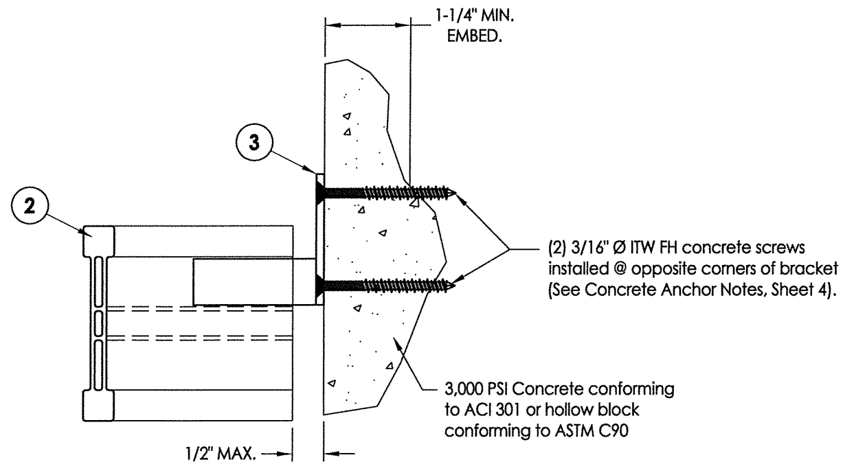
3 ANCHOR BRACKET DETAIL 3 Direct to masonry
